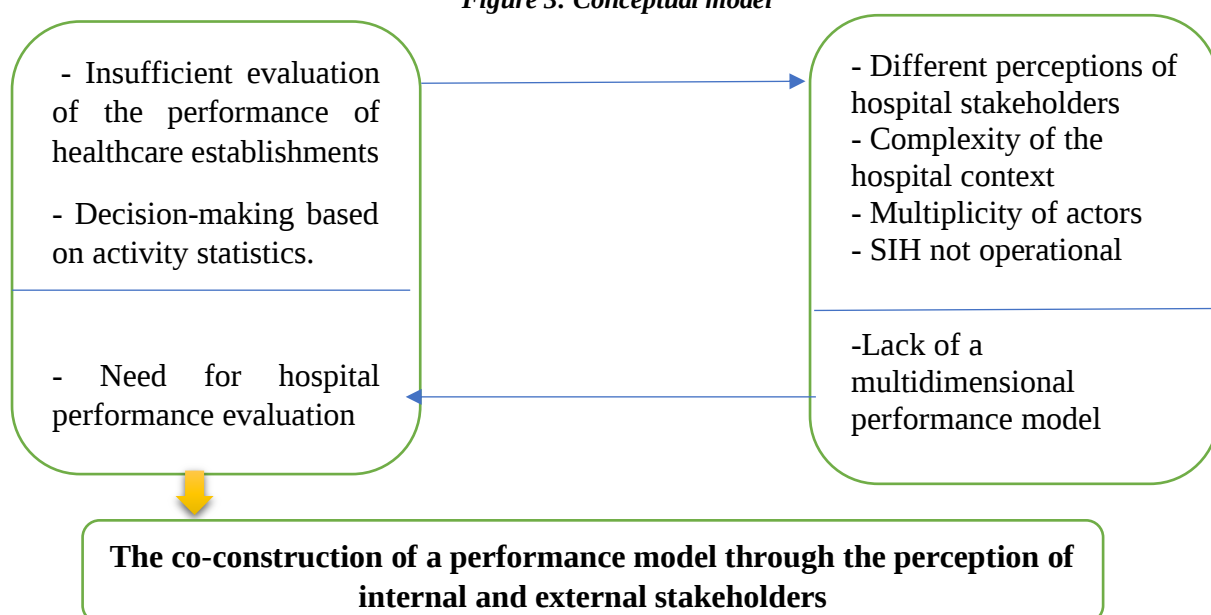
Figure 3: Conceptual model
